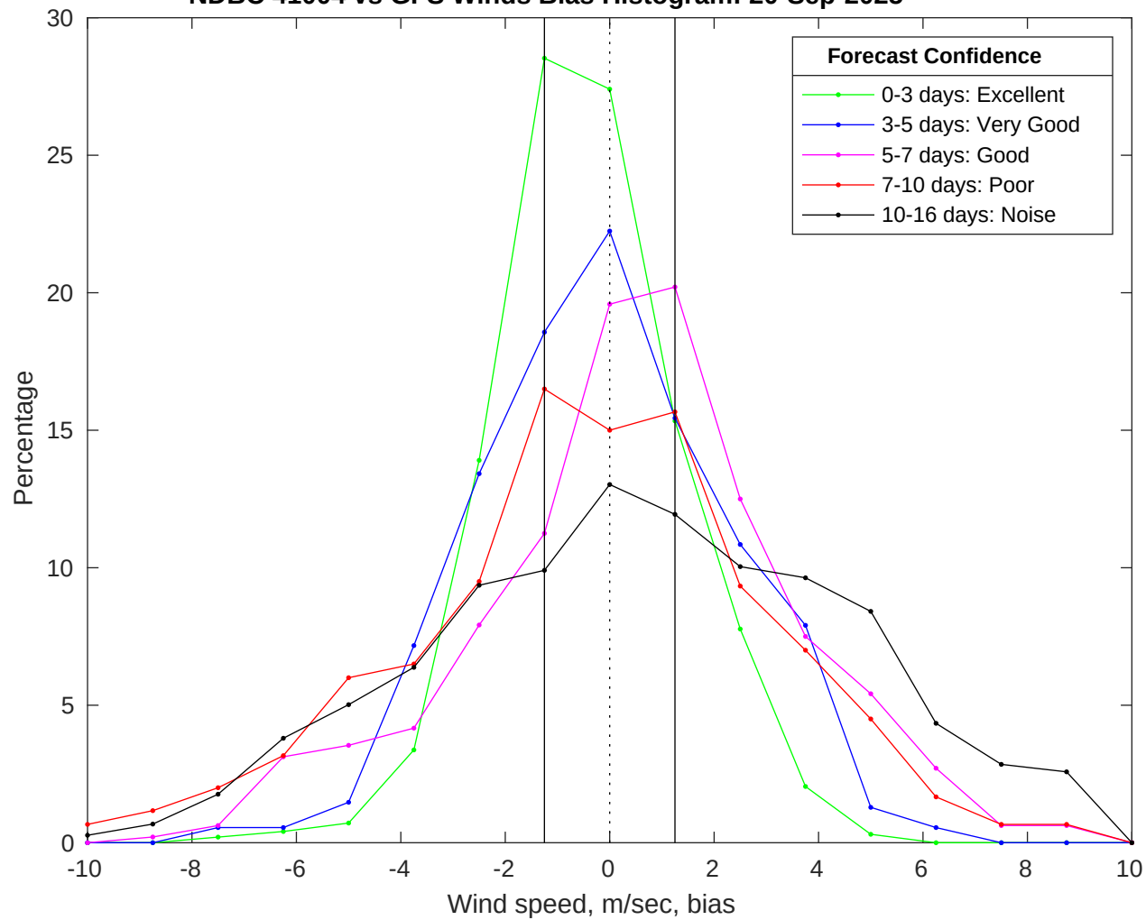
NDBC 41004 vs GFS Winds Bias Histogram: 20-Sep-2025
