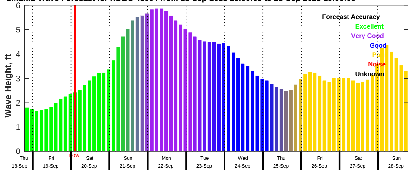
CMEMS Wave Forecast for NDBC 41004 from 18-Sep-2025 19:00:00 to 28-Sep-2025 19:00:00
