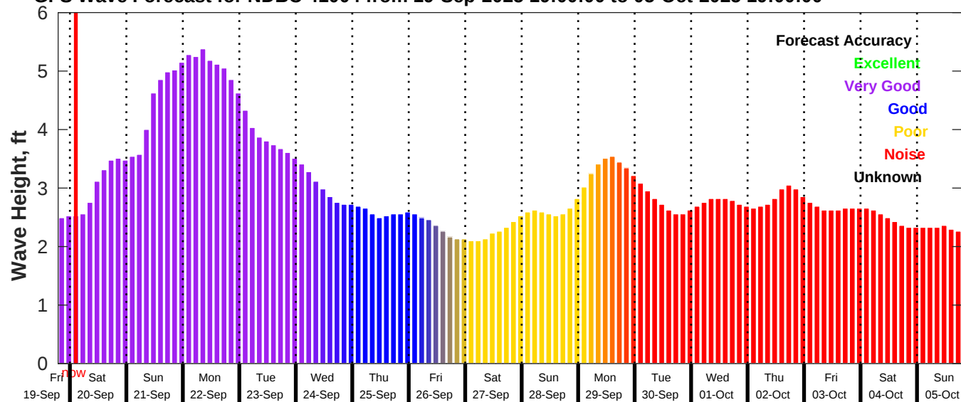
GFS Wave Forecast for NDBC 41004 from 19-Sep-2025 19:00:00 to 05-Oct-2025 19:00:00
