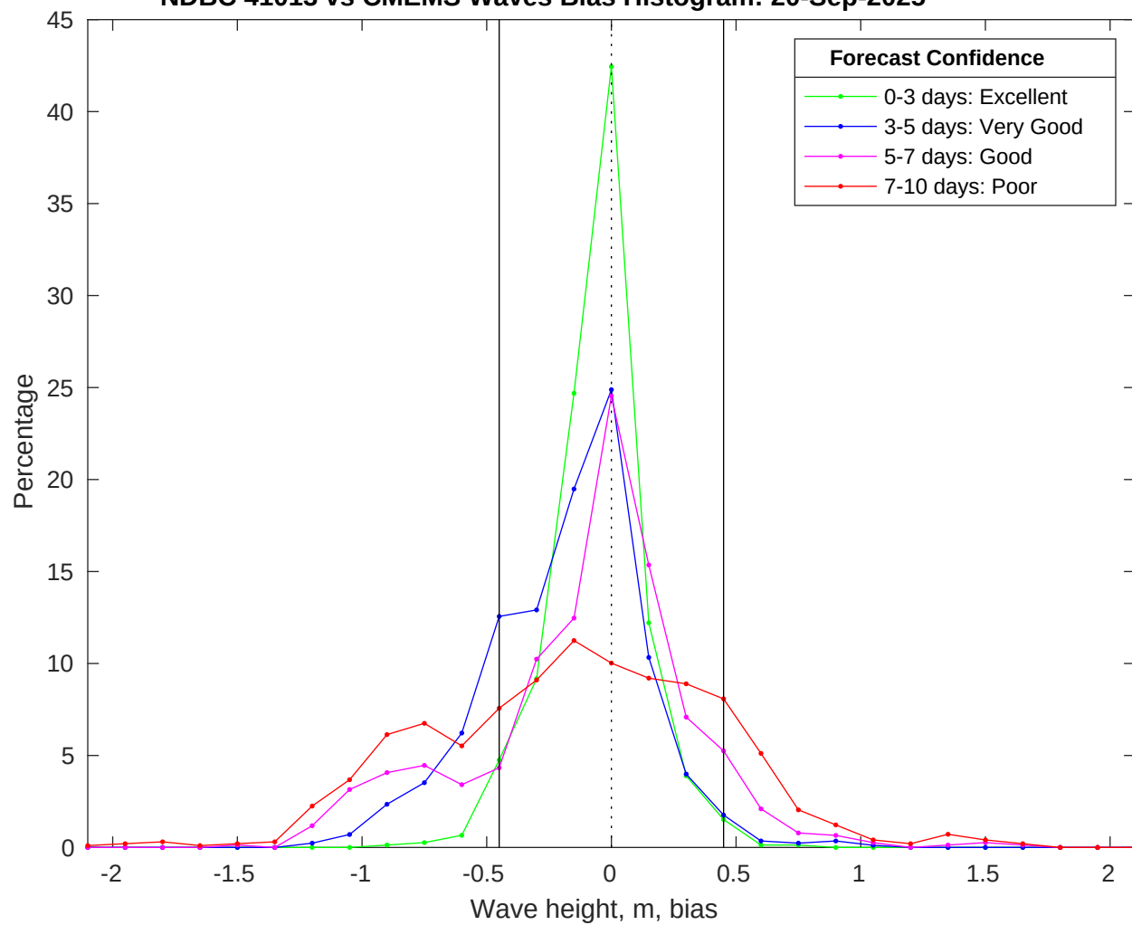
NDBC 41013 vs CMEMS Waves Bias Histogram: 20-Sep-2025
