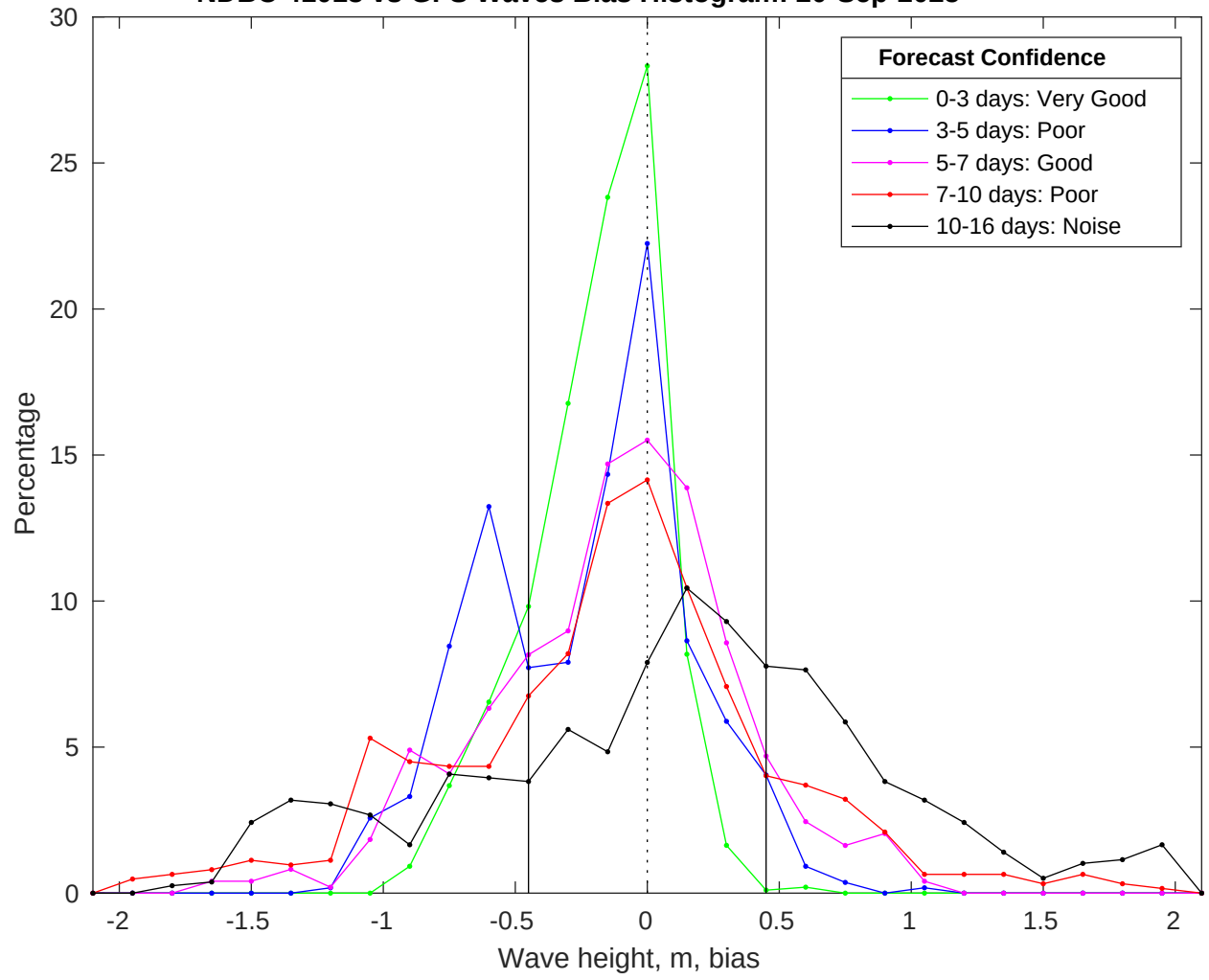
NDBC 41013 vs GFS Waves Bias Histogram: 20-Sep-2025
