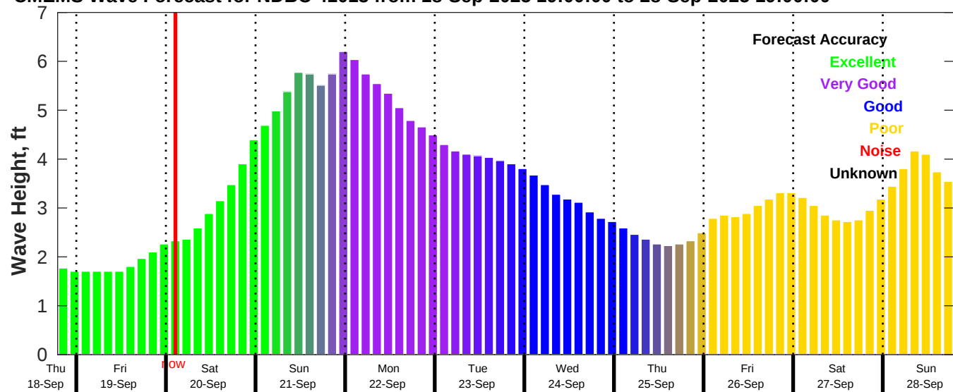
CMEMS Wave Forecast for NDBC 41013 from 18-Sep-2025 19:00:00 to 28-Sep-2025 19:00:00
