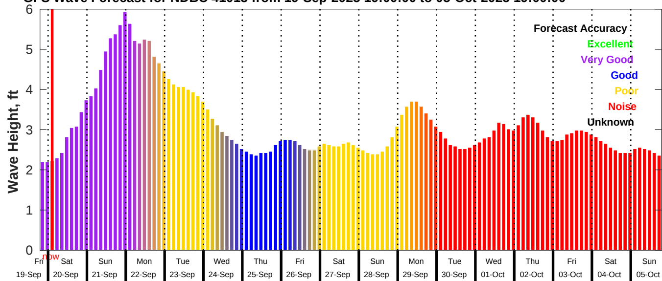
GFS Wave Forecast for NDBC 41013 from 19-Sep-2025 19:00:00 to 05-Oct-2025 19:00:00
