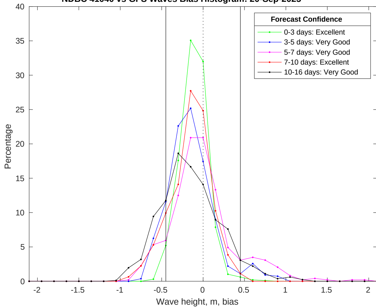
NDBC 41040 vs GFS Waves Bias Histogram: 20-Sep-2025
