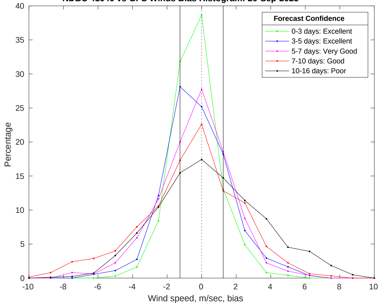
NDBC 41040 vs GFS Winds Bias Histogram: 20-Sep-2025
