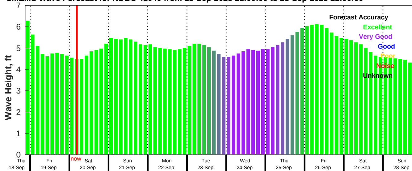
CMEMS Wave Forecast for NDBC 41040 from 18-Sep-2025 21:00:00 to 28-Sep-2025 21:00:00
