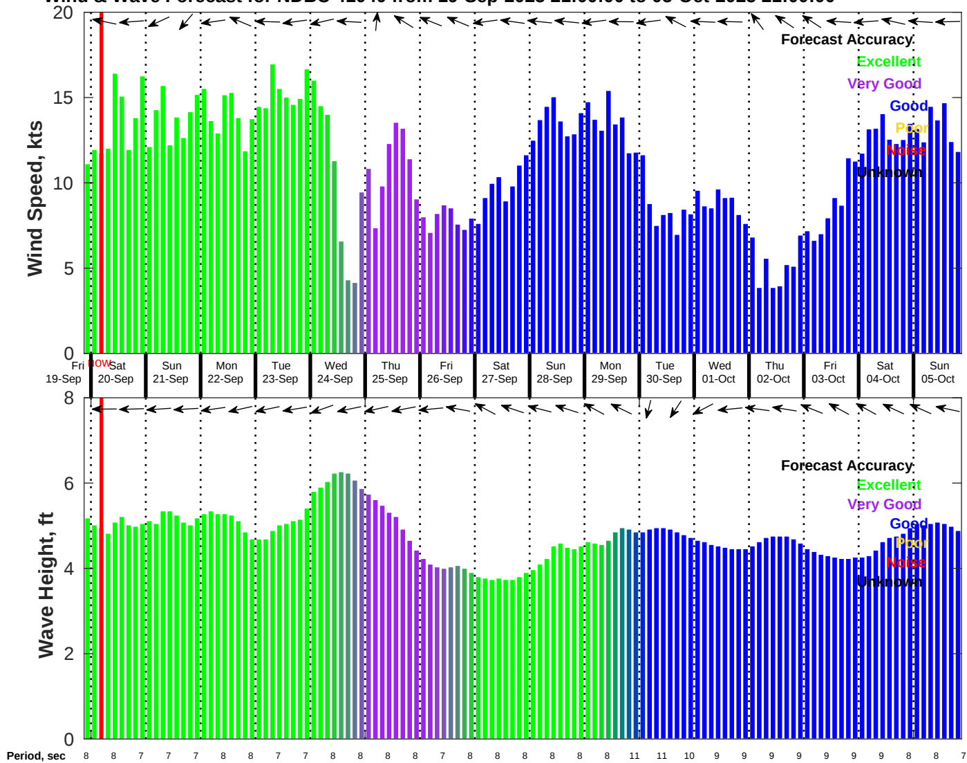
Wind & Wave Forecast for NDBC 41040 from 19-Sep-2025 21:00:00 to 05-Oct-2025 21:00:00
