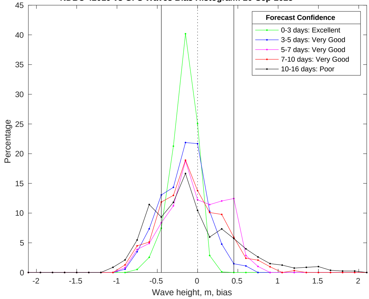
NDBC 42019 vs GFS Waves Bias Histogram: 20-Sep-2025
