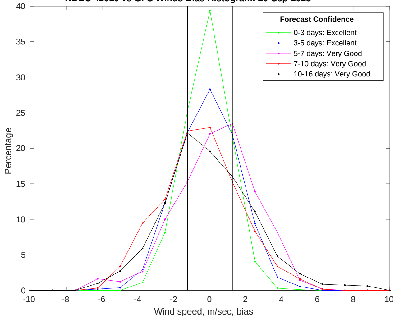
NDBC 42019 vs GFS Winds Bias Histogram: 20-Sep-2025
