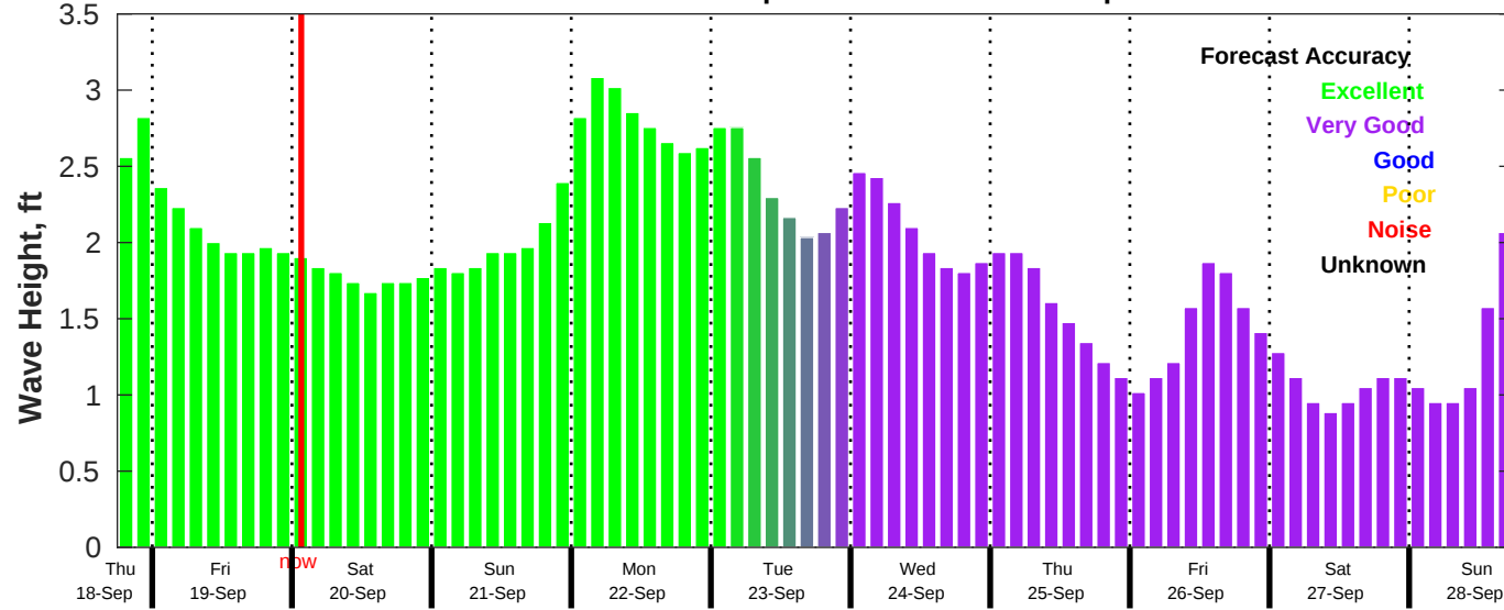
CMEMS Wave Forecast for NDBC 42019 from 18-Sep-2025 18:00:00 to 28-Sep-2025 18:00:00
