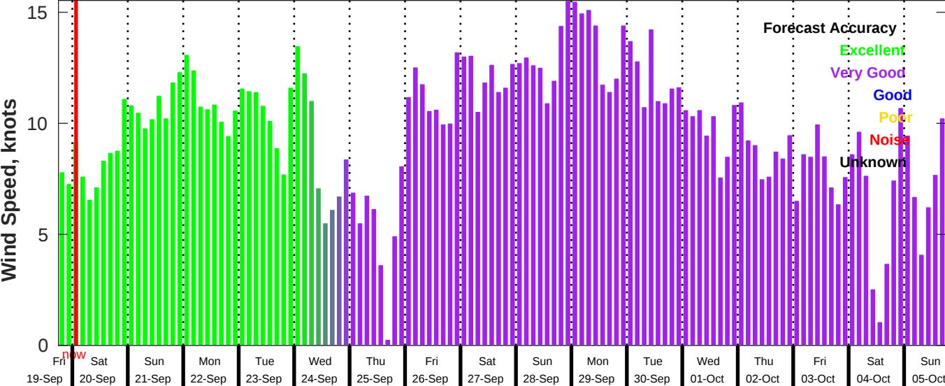
GFS Wind Speed Forecast for NDBC 42019 from 19-Sep-2025 18:00:00 to 05-Oct-2025 18:00:00
