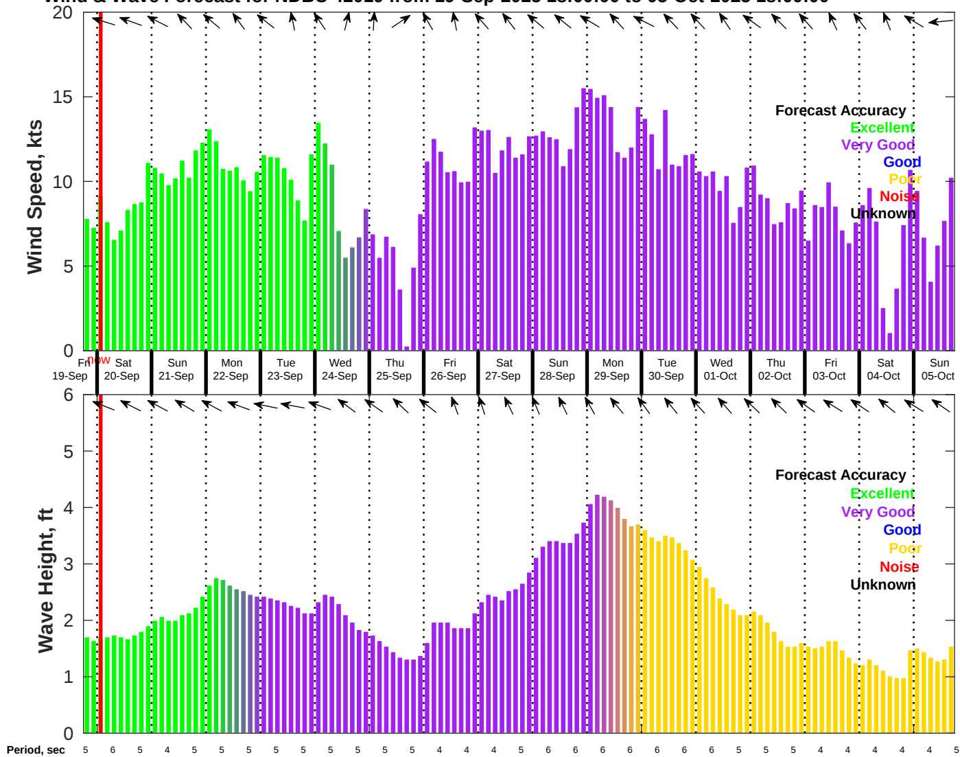
Wind & Wave Forecast for NDBC 42019 from 19-Sep-2025 18:00:00 to 05-Oct-2025 18:00:00
