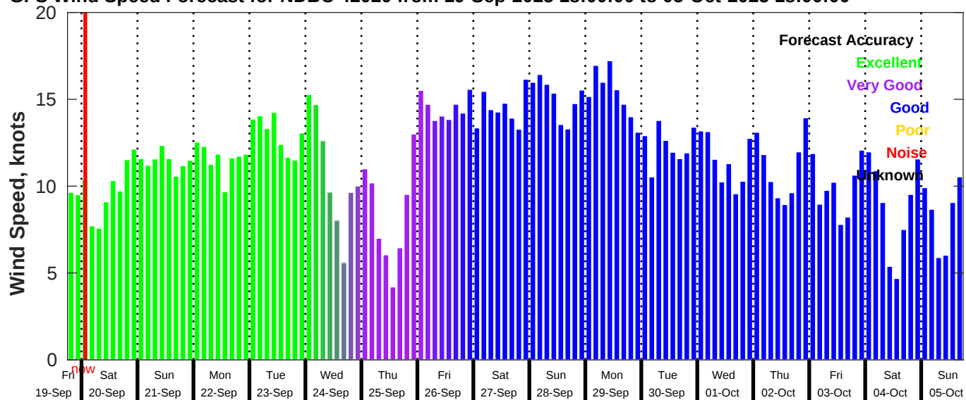
GFS Wind Speed Forecast for NDBC 42020 from 19-Sep-2025 18:00:00 to 05-Oct-2025 18:00:00
