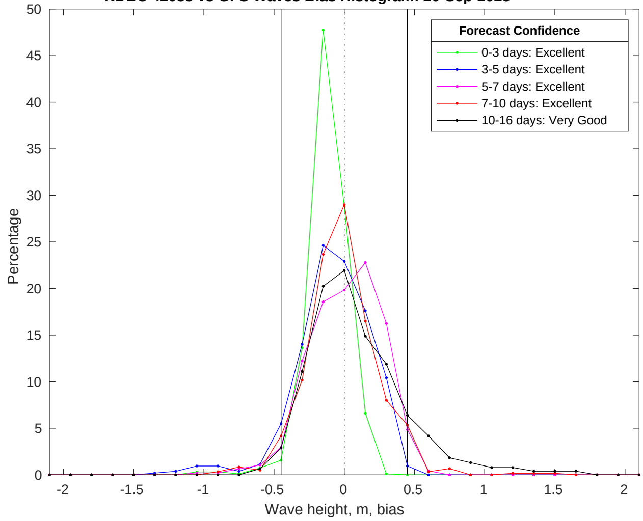
NDBC 42035 vs GFS Waves Bias Histogram: 20-Sep-2025
