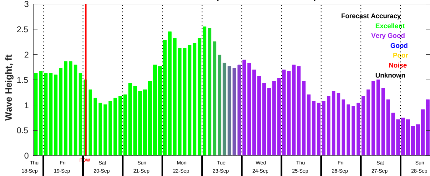
CMEMS Wave Forecast for NDBC 42035 from 18-Sep-2025 18:00:00 to 28-Sep-2025 18:00:00
