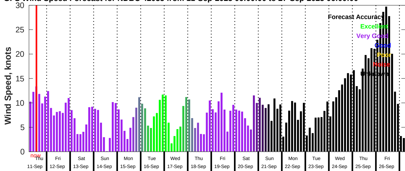
GFS Wind Speed Forecast for NDBC 42035 from 11-Sep-2025 06:00:00 to 27-Sep-2025 06:00:00
