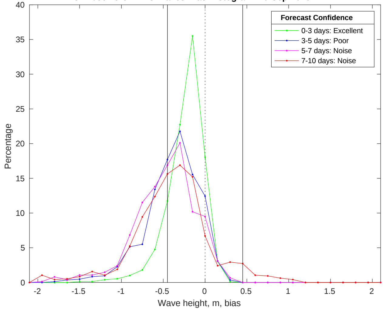
NDBC 42036 vs CMEMS Waves Bias Histogram: 20-Sep-2025
