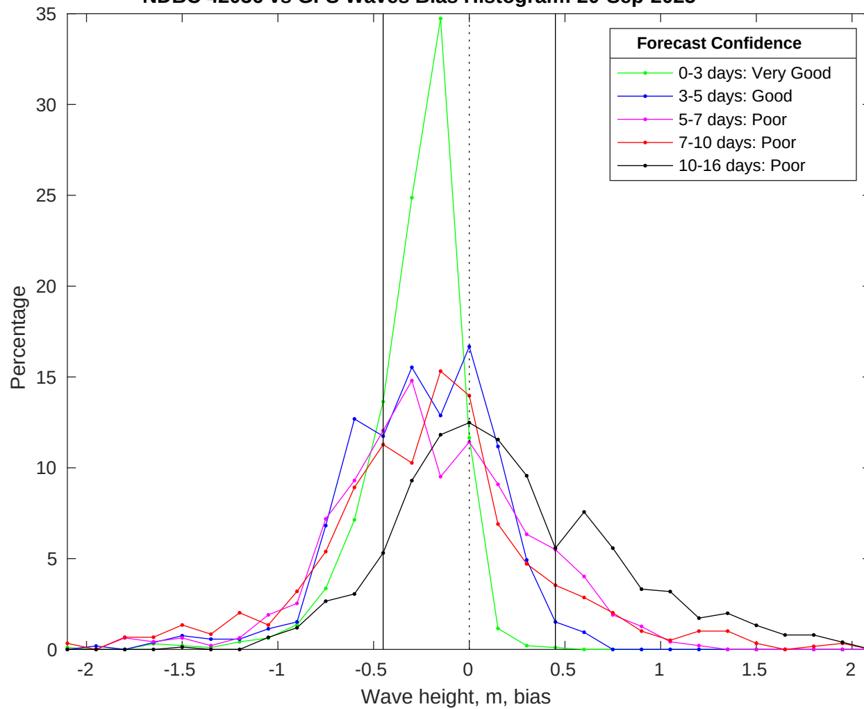
NDBC 42036 vs GFS Waves Bias Histogram: 20-Sep-2025
