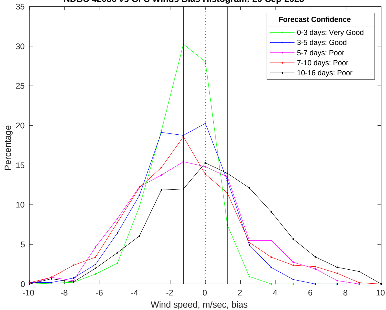
NDBC 42036 vs GFS Winds Bias Histogram: 20-Sep-2025
