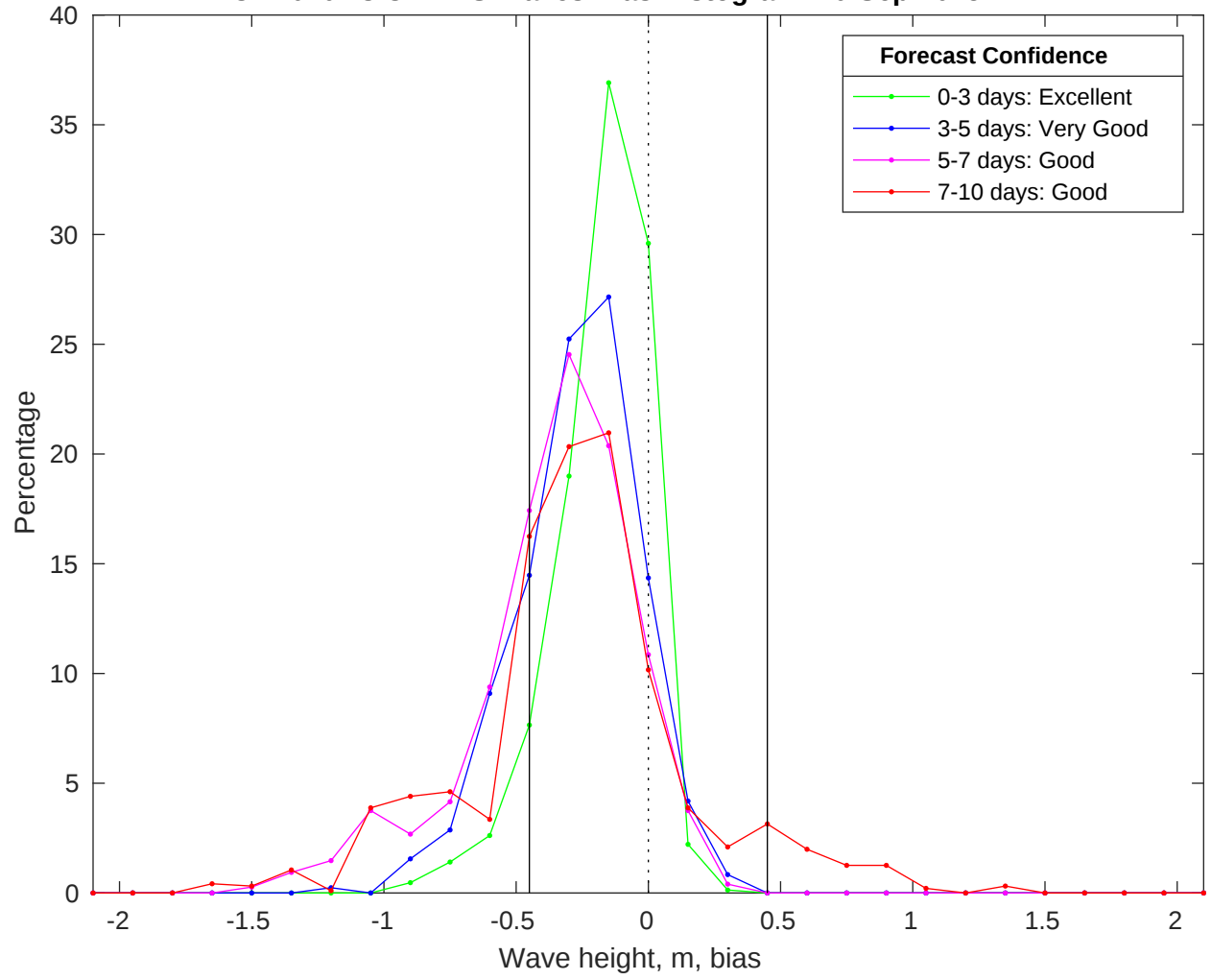
NDBC 42040 vs CMEMS Waves Bias Histogram: 20-Sep-2025
