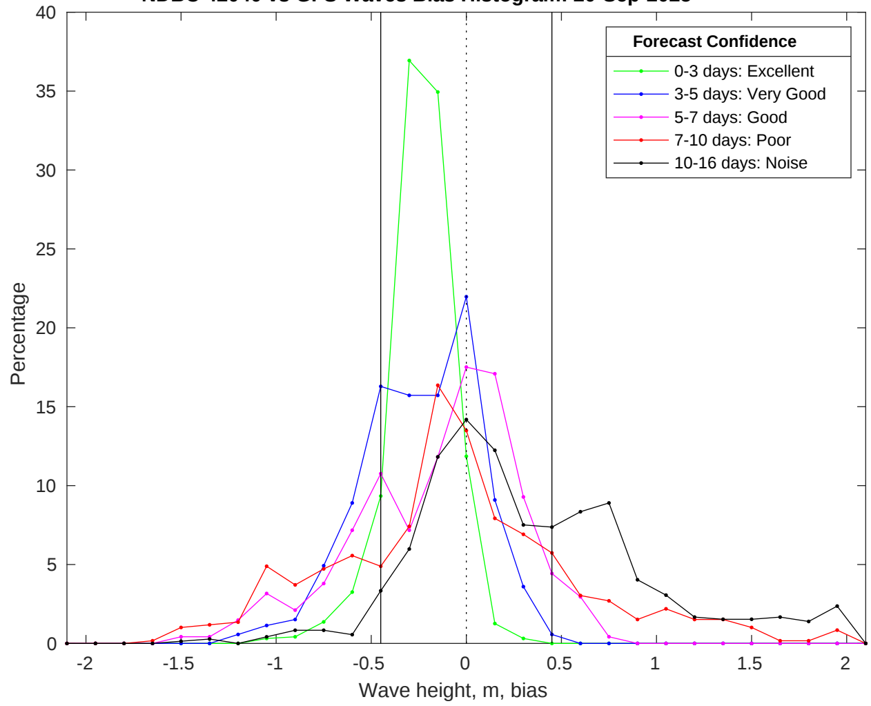
NDBC 42040 vs GFS Waves Bias Histogram: 20-Sep-2025
