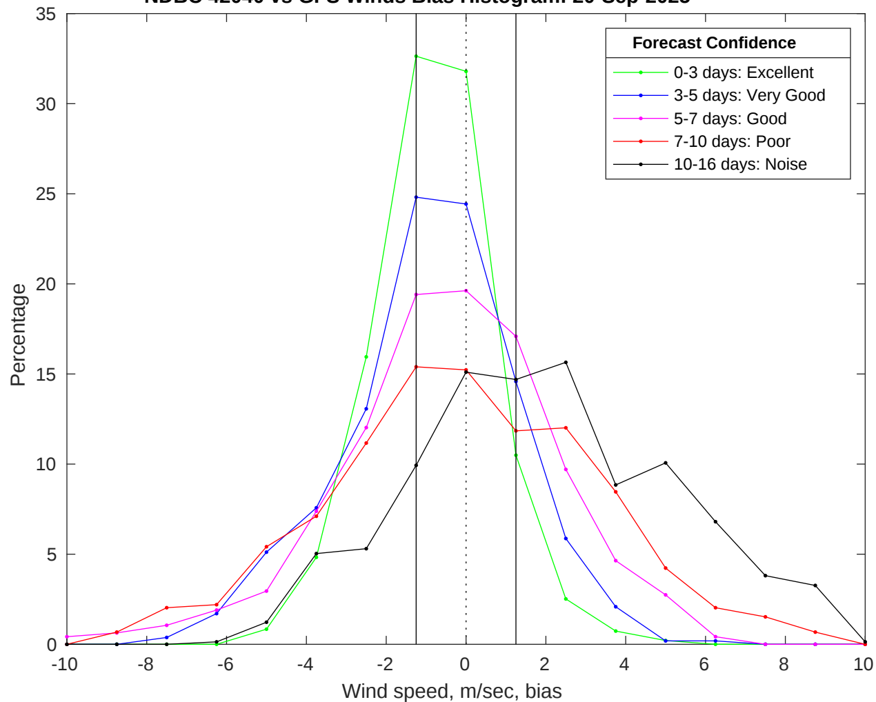
NDBC 42040 vs GFS Winds Bias Histogram: 20-Sep-2025
