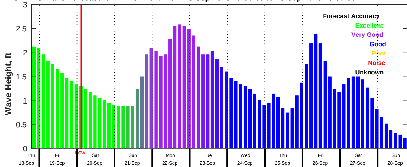
CMEMS Wave Forecast for NDBC 42040 from 18-Sep-2025 19:00:00 to 28-Sep-2025 19:00:00
