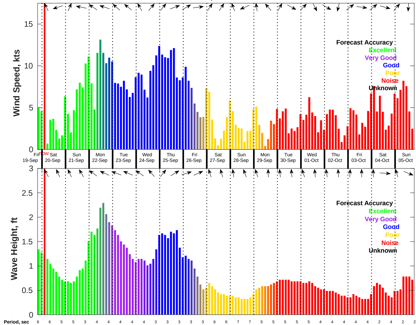
Wind & Wave Forecast for NDBC 42040 from 19-Sep-2025 19:00:00 to 05-Oct-2025 19:00:00
