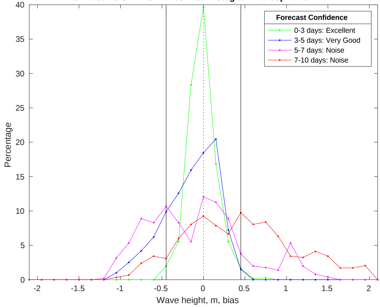
NDBC 44008 vs CMEMS Waves Bias Histogram: 20-Sep-2025
