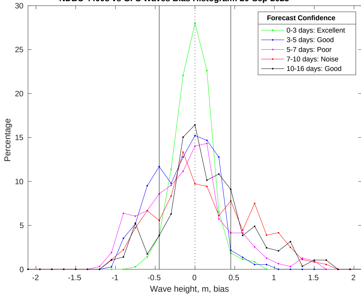
NDBC 44008 vs GFS Waves Bias Histogram: 20-Sep-2025
