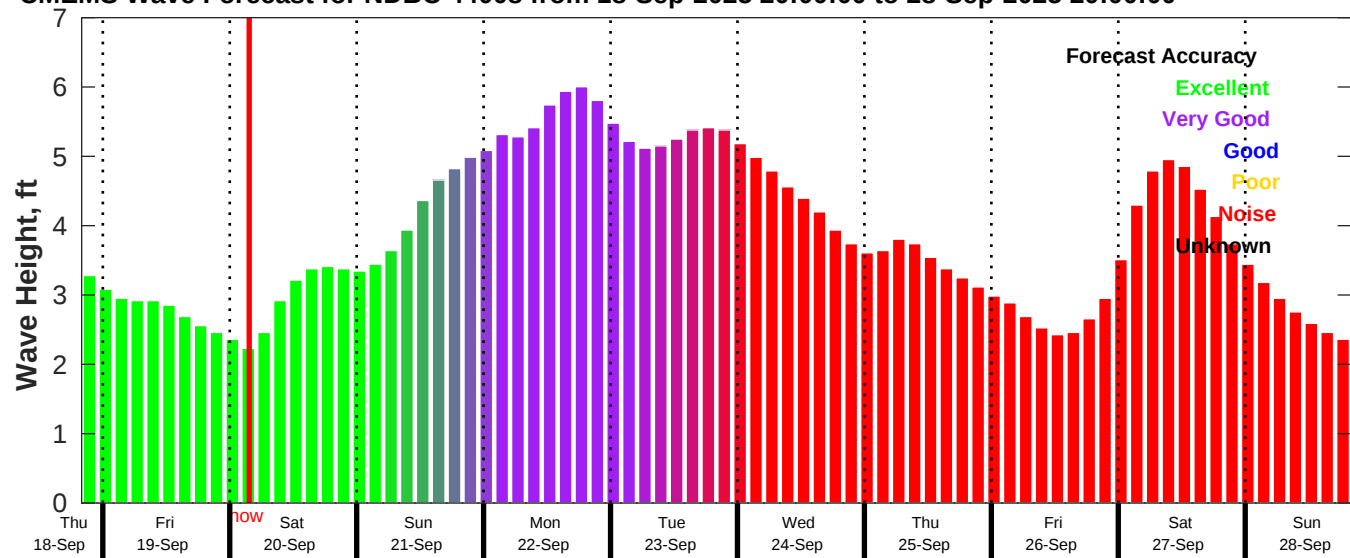
CMEMS Wave Forecast for NDBC 44008 from 18-Sep-2025 20:00:00 to 28-Sep-2025 20:00:00
