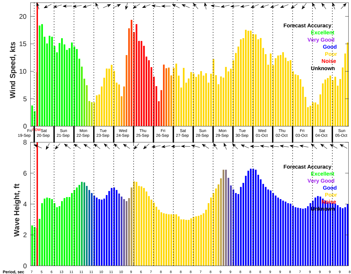
Wind & Wave Forecast for NDBC 44008 from 19-Sep-2025 20:00:00 to 05-Oct-2025 20:00:00
