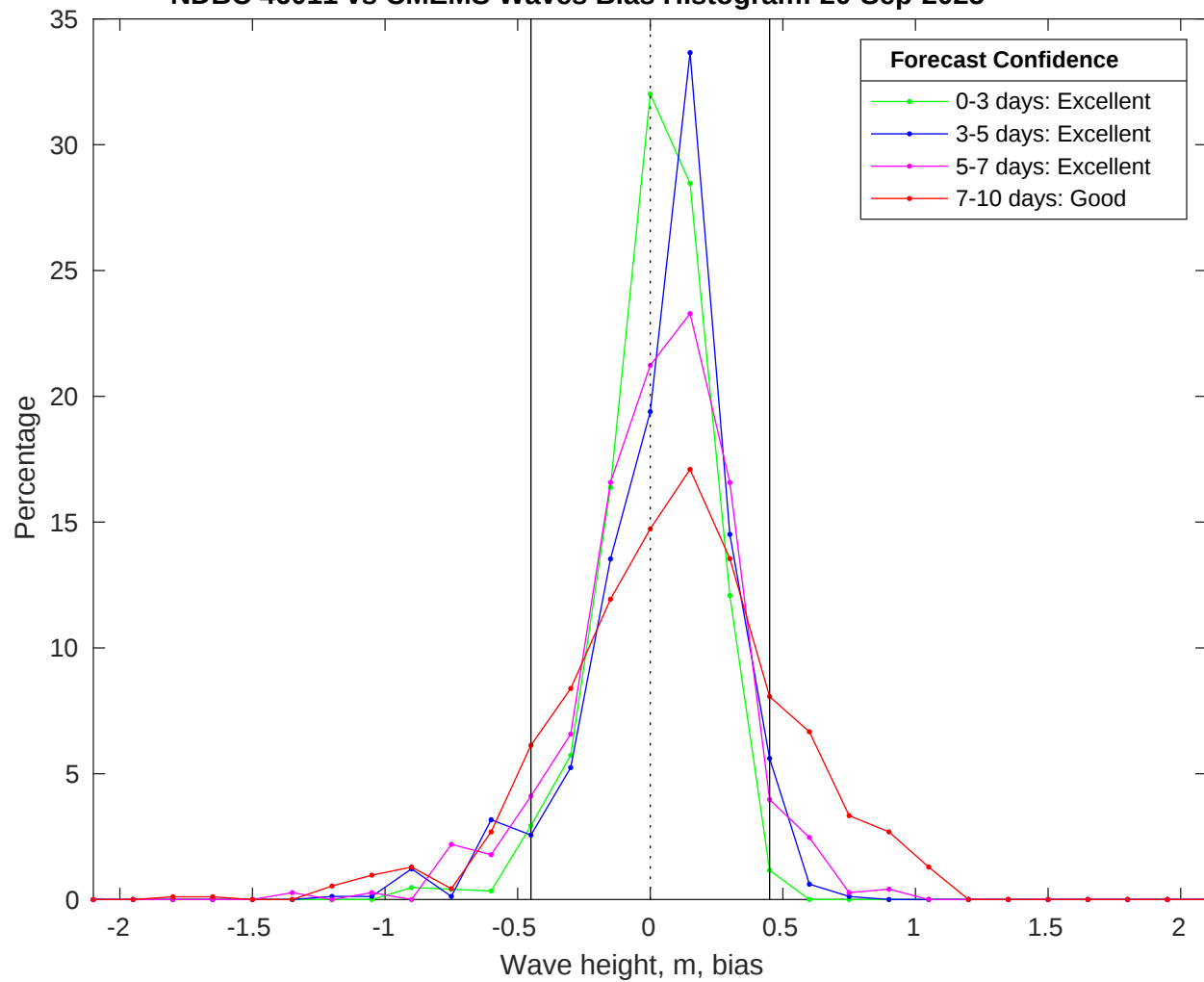
NDBC 46011 vs CMEMS Waves Bias Histogram: 20-Sep-2025
