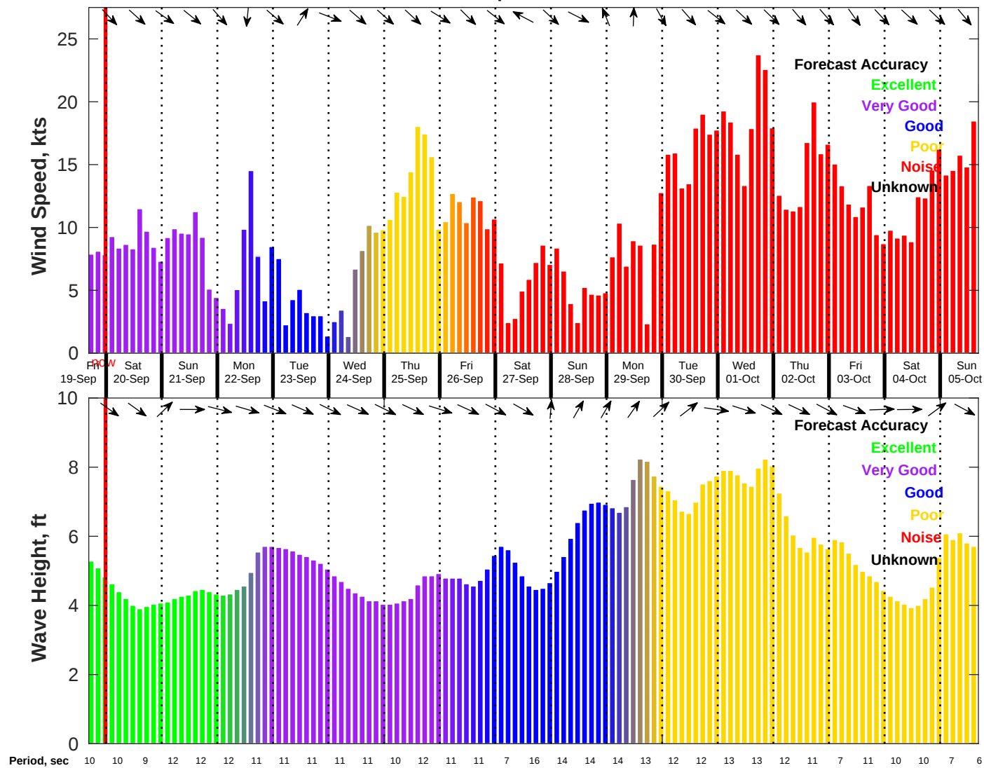
Wind & Wave Forecast for NDBC 46011 from 19-Sep-2025 16:00:00 to 05-Oct-2025 16:00:00
