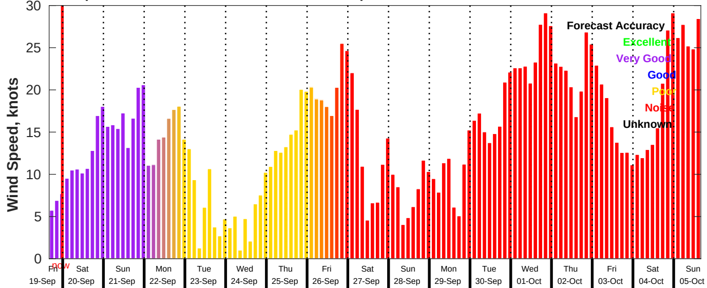
GFS Wind Speed Forecast for NDBC 46028 from 19-Sep-2025 16:00:00 to 05-Oct-2025 16:00:00
