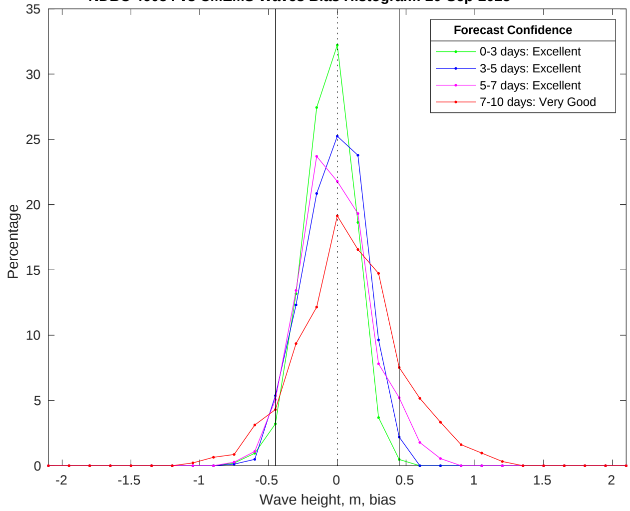
NDBC 46054 vs CMEMS Waves Bias Histogram: 20-Sep-2025
