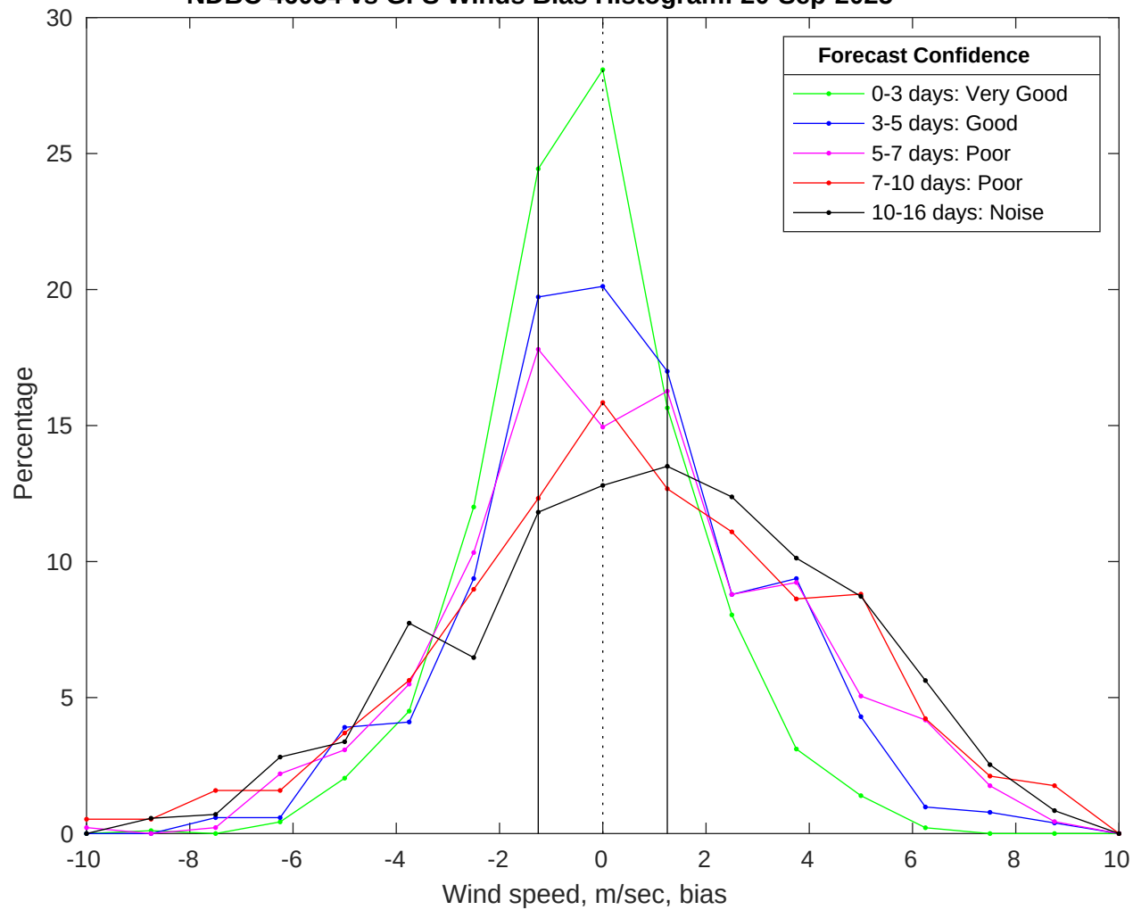
NDBC 46054 vs GFS Winds Bias Histogram: 20-Sep-2025
