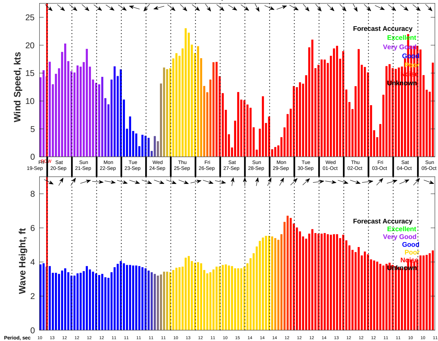
Wind & Wave Forecast for NDBC 46054 from 19-Sep-2025 16:00:00 to 05-Oct-2025 16:00:00
