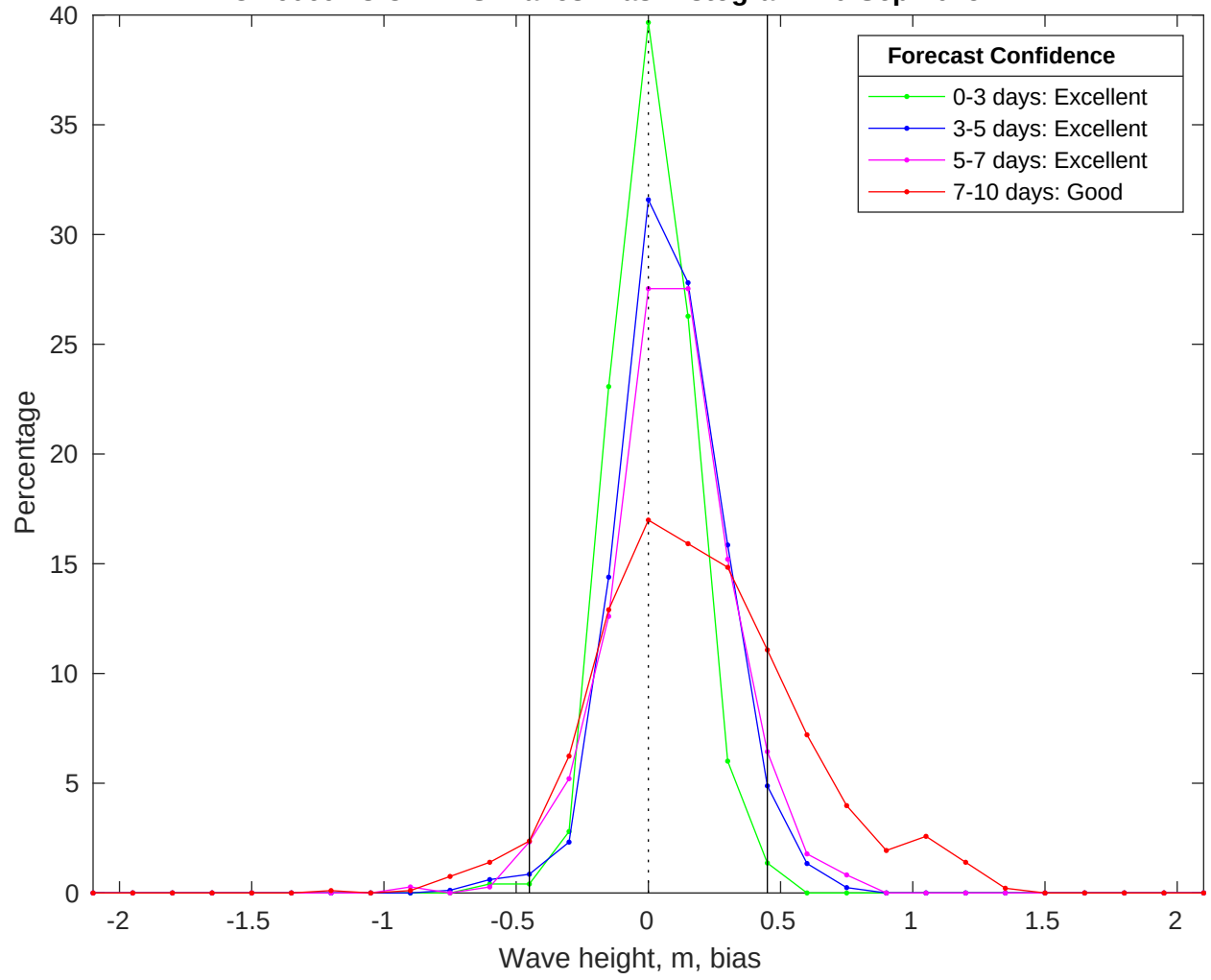
NDBC 46069 vs CMEMS Waves Bias Histogram: 20-Sep-2025
