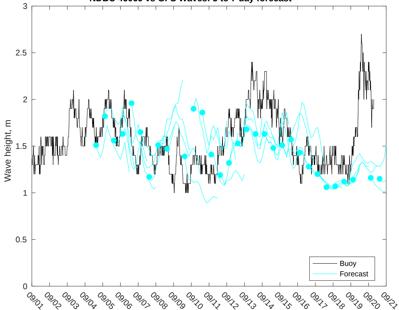
NDBC 46069 vs GFS Waves: 5 to 7 day forecast
