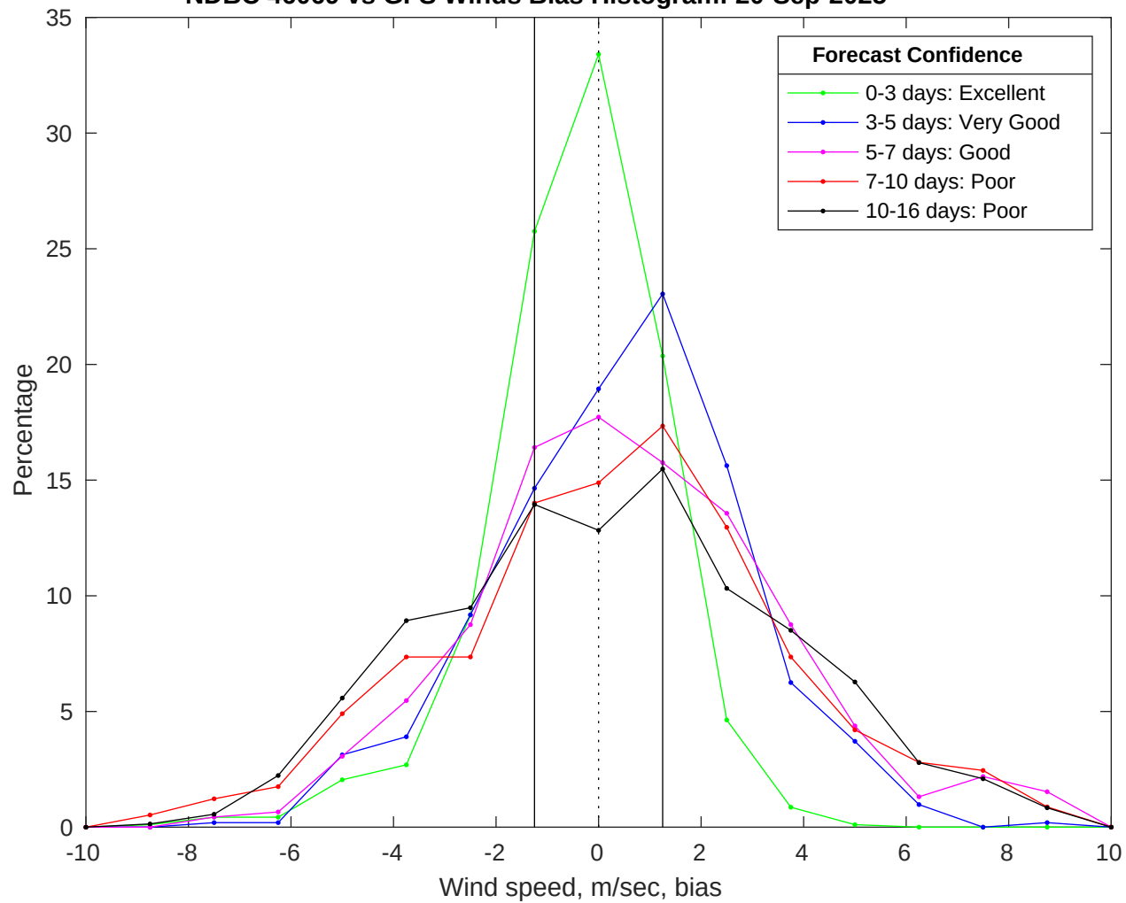
NDBC 46069 vs GFS Winds Bias Histogram: 20-Sep-2025
