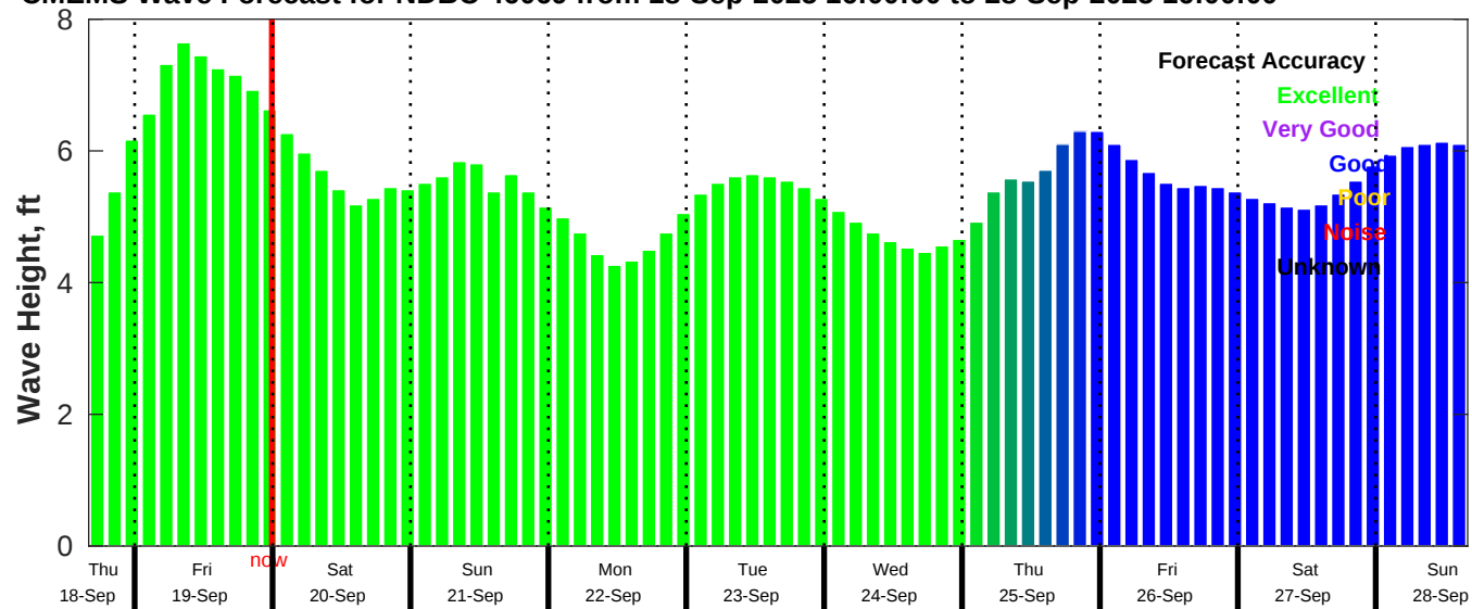
CMEMS Wave Forecast for NDBC 46069 from 18-Sep-2025 16:00:00 to 28-Sep-2025 16:00:00
