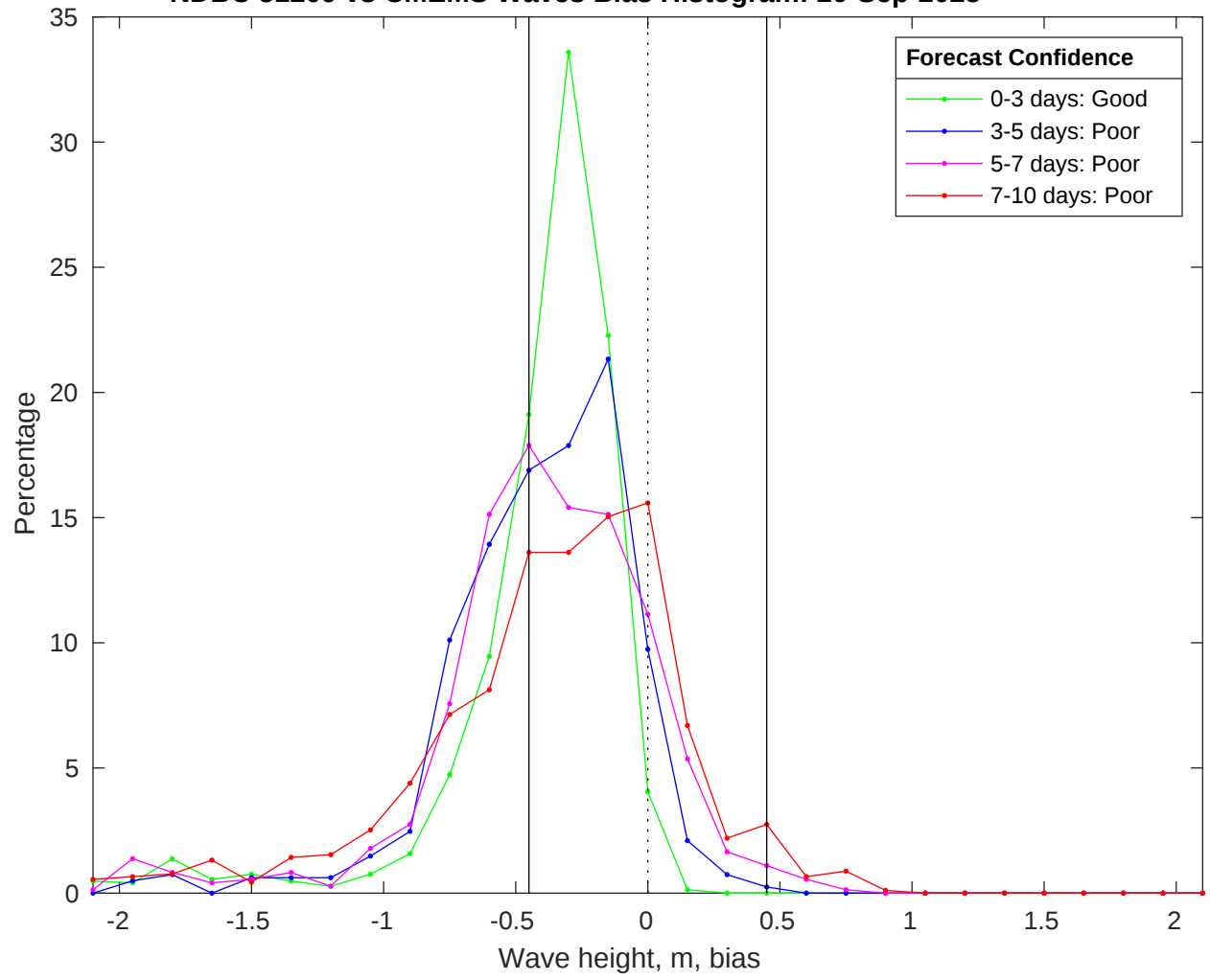
NDBC 51209 vs CMEMS Waves Bias Histogram: 20-Sep-2025
