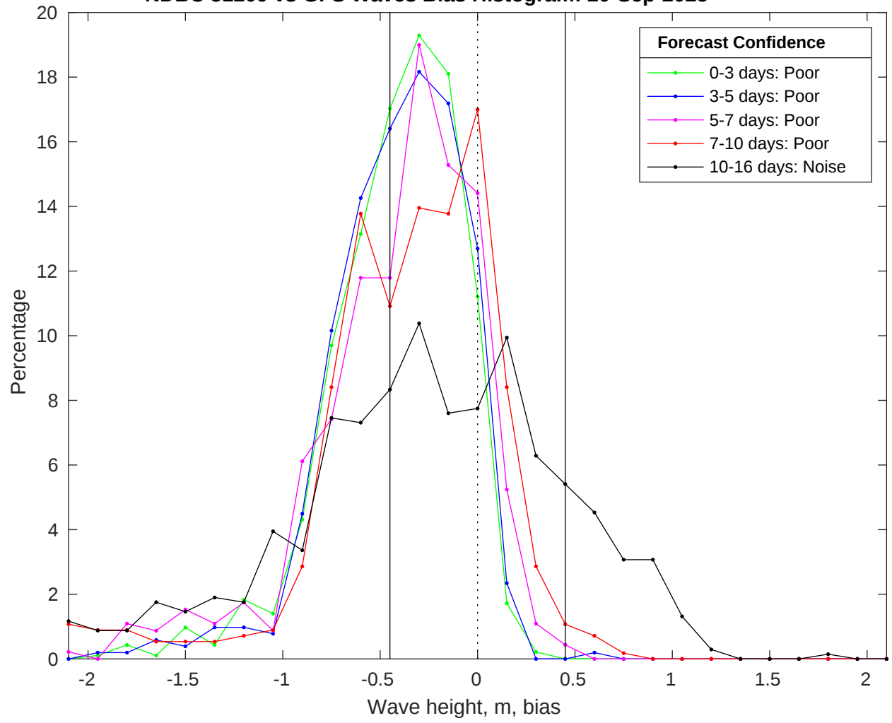
NDBC 51209 vs GFS Waves Bias Histogram: 20-Sep-2025
