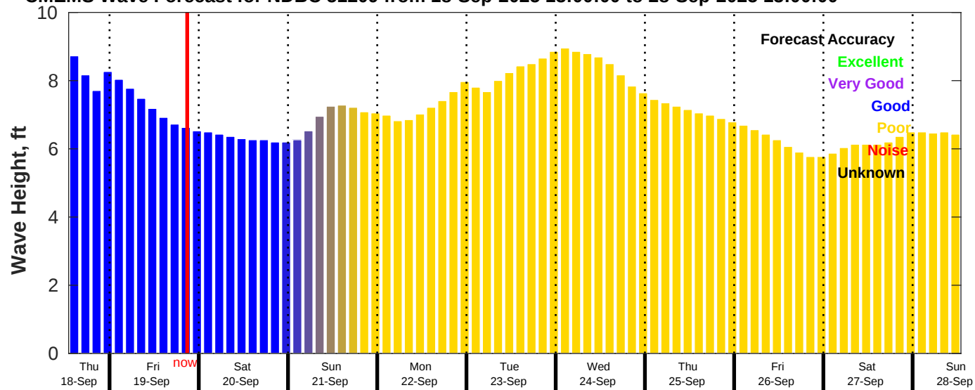
CMEMS Wave Forecast for NDBC 51209 from 18-Sep-2025 13:00:00 to 28-Sep-2025 13:00:00
