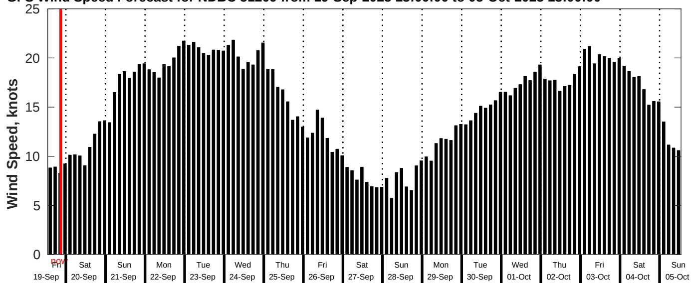
GFS Wind Speed Forecast for NDBC 51209 from 19-Sep-2025 13:00:00 to 05-Oct-2025 13:00:00
