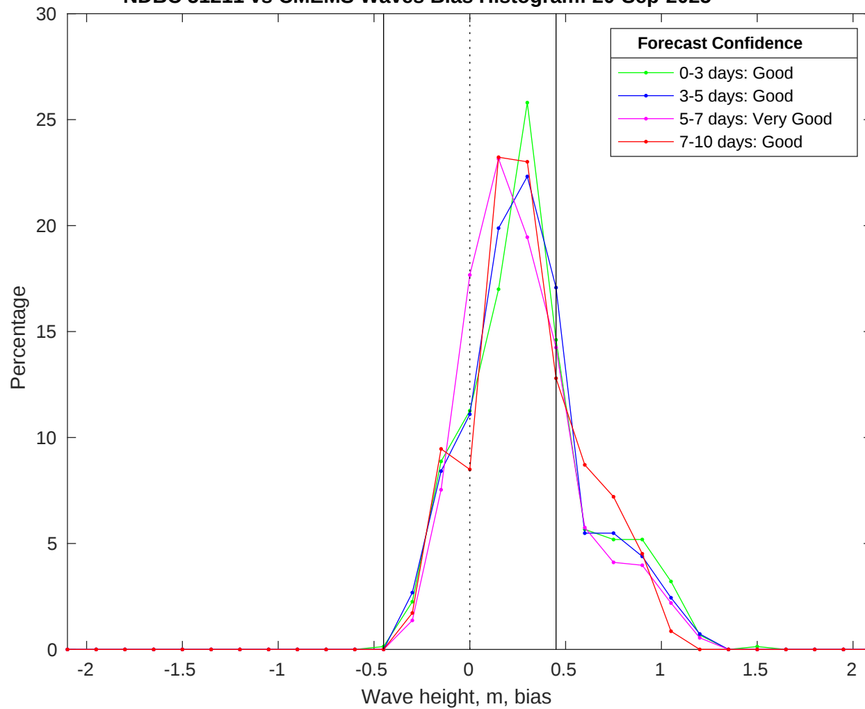
NDBC 51211 vs CMEMS Waves Bias Histogram: 20-Sep-2025
