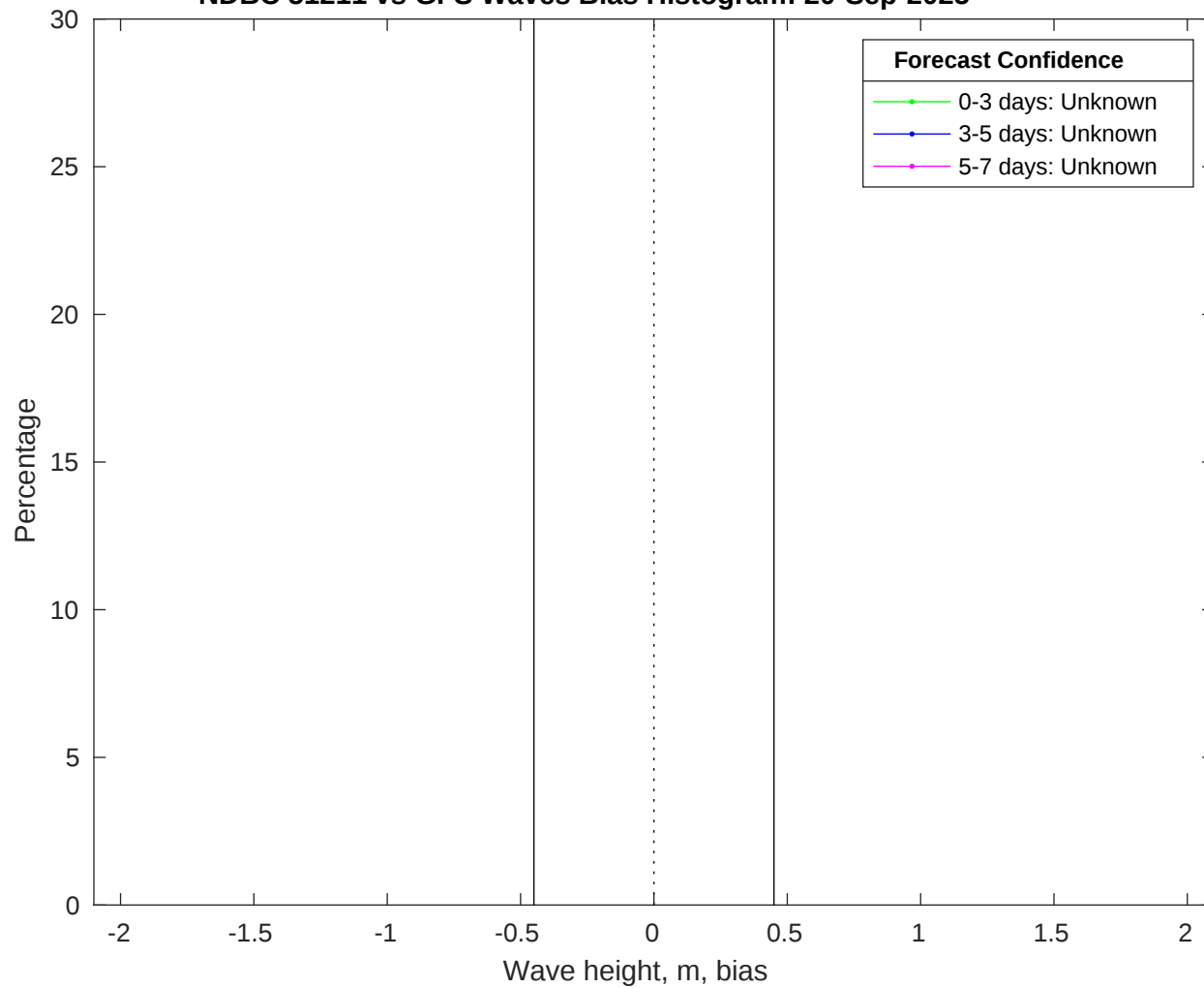
NDBC 51211 vs GFS Waves Bias Histogram: 20-Sep-2025
