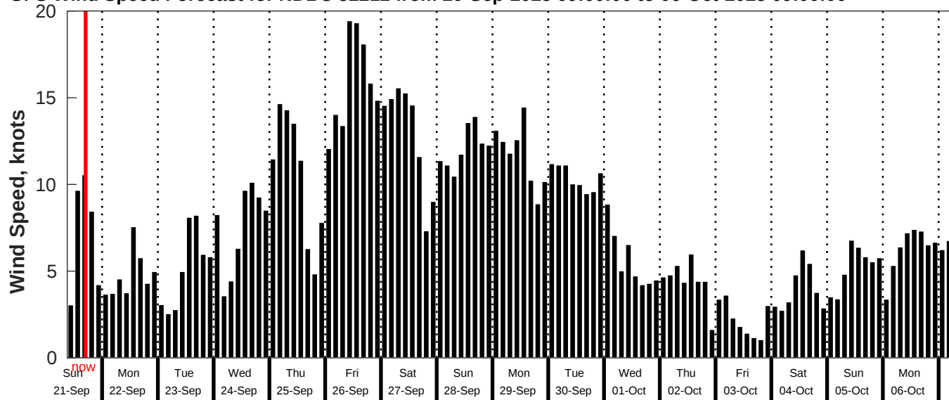
GFS Wind Speed Forecast for NDBC 52212 from 20-Sep-2025 09:00:00 to 06-Oct-2025 09:00:00
