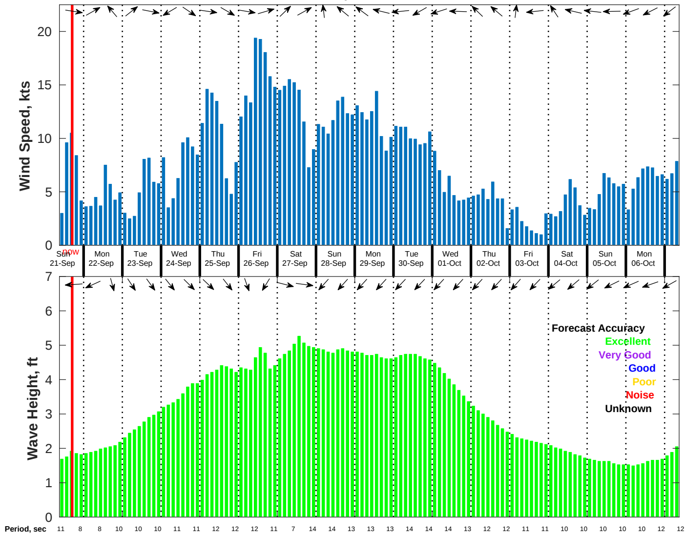
Wind & Wave Forecast for NDBC 52212 from 20-Sep-2025 09:00:00 to 06-Oct-2025 09:00:00
